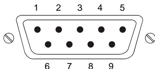
Pin assignment of FCBI module
